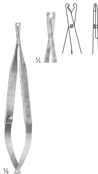
03-114 BIEMER Vein Scissor Size: 130 mm 03-115 Size: 160 mm
