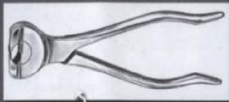
11-322-16 Martin "Diamant" (16 cm / 6 1/4") Soft wires up to 2.2mm Ø Hard wires up to 2.0mm Ø
